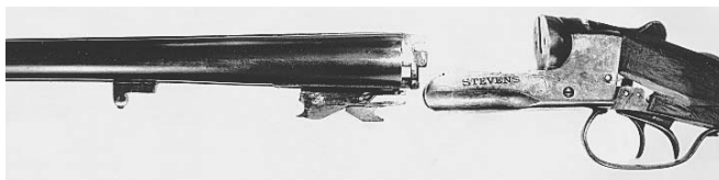
Stevens Model 330 early fork-type cocking lever
