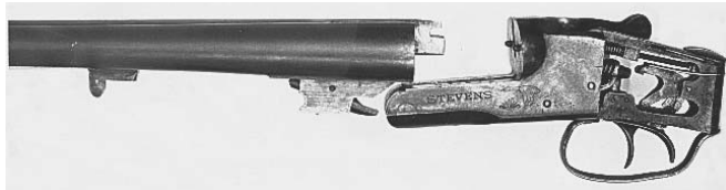
Stevens Model 330 late spade-type cocking lever
